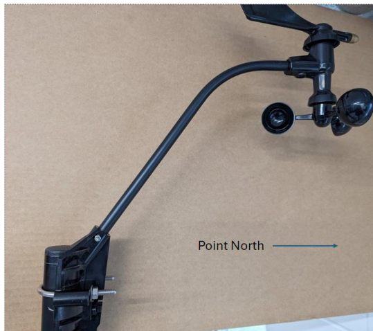
Install MET ( Notch must point North)
